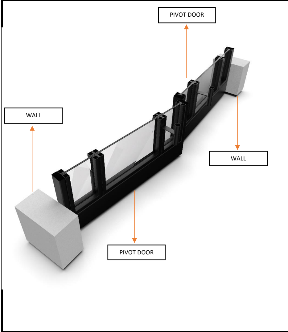
Shows double pivot door assembly
